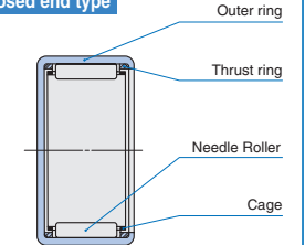
Caged type with two seals
