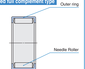
Grease retained full complement type
