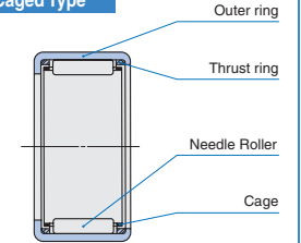
Standard Caged Type
